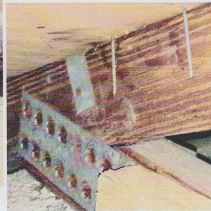
Toe Nailed (Metal connectors that do not meet the minimum requirements)
